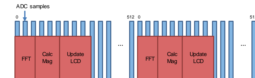
Figure 4. Timing Diagram
