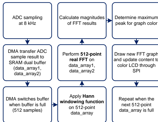
Figure 3. Application Flow Chart
